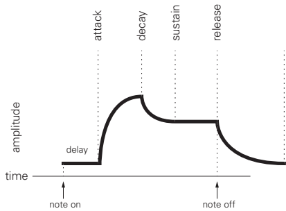
A typical five-stage, DADSR envelope
